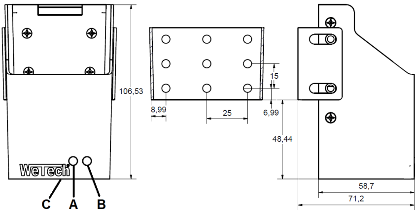
Schematic drawing WTC642
